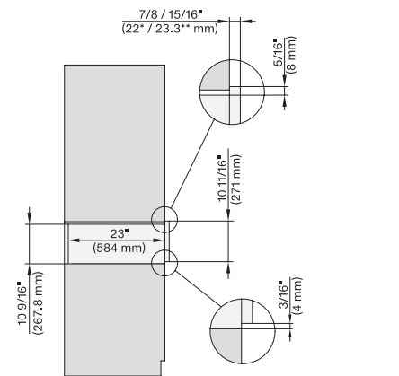
side view 30 inch Proud ESW30, installation drawing, NA
