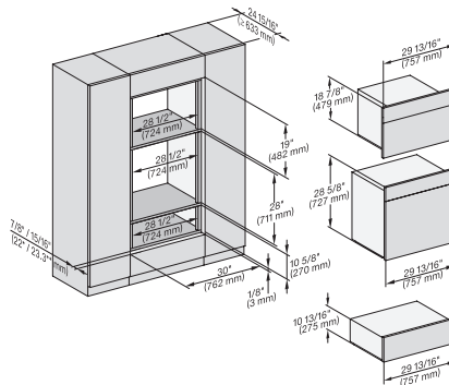
H 656x, H 6x60, DGC686x+EBA 6808, H 6x70, DGC 676x, DGC7x7x. EBA7868, H 7xxx, Fitti Combi, Install drawi, Flush inset, NA
