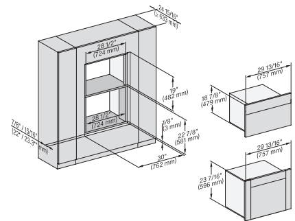
H 6x80 BP, H 6x70 BM, H 6x80-2BP, DGC7x7x, H7xxx Fitting Combi, Installation drawing, Flush inset, NA
