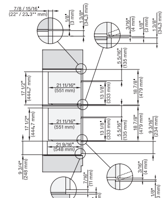
H 6x70 BM, ESW 6x85, DGC7xxx, H7x7x, ESW 7x70 Combi, installation drawing, Flush inset, Flush inset, NA
