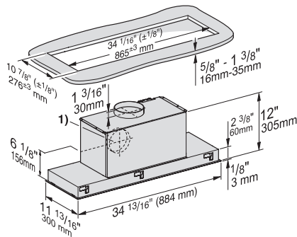
DA2390 (Installation drawing) – US
