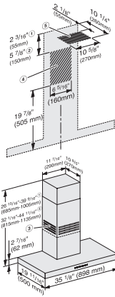
PUR98W, DAP1927 (Installation drawing) – USA/CDN
