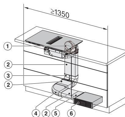
KMDA7272-1FL/FR, KMDA7473-1FL/FL MattFinish/FR, KMDA7272FL/FR, KMDA7473FL/FR – Installation variant 4 Circulating air
