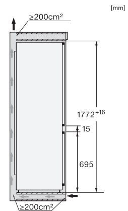
KFN7795D, KFN7795C, KFNS7795D, side view
