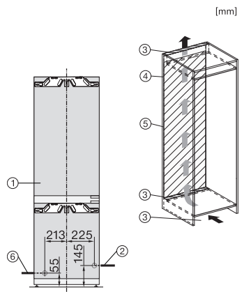
KFN7795D, KFN7795C, KFNS7795D, installation
