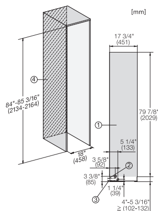
F2413Vi, F2411Vi, F2411SF, F2461Vi, F2411Vi, F2411SF, installation, MasterCool, installation drawings
