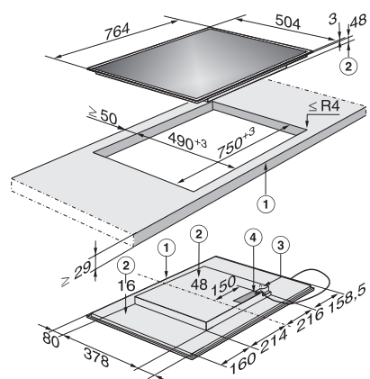
KM 6307, KM 6347 PowerFlex (Installation drawing)
