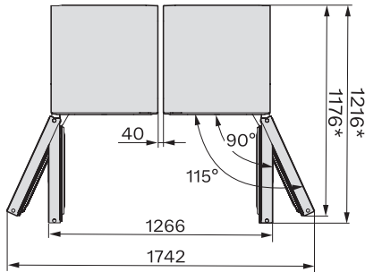
K4373ED, KS4383ED, KS4383 C ED, KS4783 bb Blackboard, KS4887DD, installation
