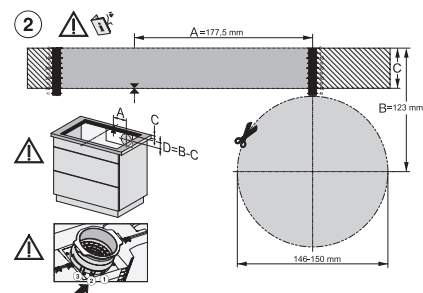
KMDA7272-1FL/FR, KMDA7473-1FL/FR, KMDA7272FL/FR, KMDA7473FL/FR – Installation variant 11 Exhaust air
