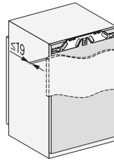
K7364D, K7343D, K7344D, K7344C, K7373B, K7374D, built-in (footnote*) (installation drawings)
