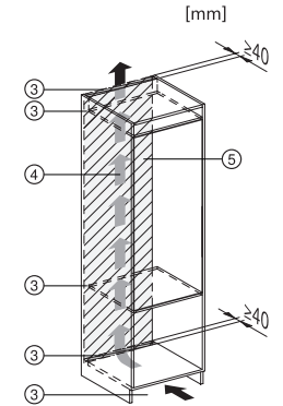
K7313D, K7313F, K7314E, K7314F, K7303F, K7303D, K7304F, K7304E, installation (footnote*) (installation drawings)
