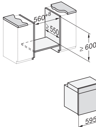
H226x-1B/BP/E/EP/1/IP, H2x6xB/BP, H7x6xB/BP/BPX, installation drawings
