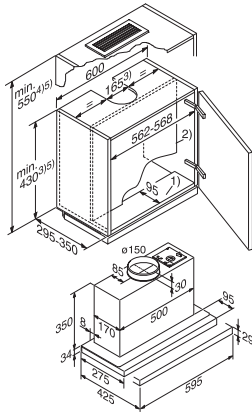
DA 3360, DA 3366 (Installation drawing)
