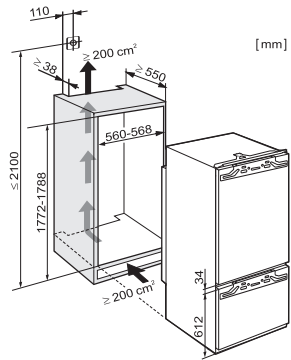
K9726iF, K9759iDF (Installation drawing)
