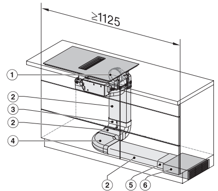
KMDA7676-1FL, KMDA7876-1FL, KMDA7676FL, KMDA7876FL - Installation variant 13 Circulating air
