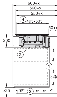
KMDA7272-1FL, KMDA7473-1FL/FL MattFinish, KMDA7272FL, KMDA7473FL - Side view flush+X, Plug&Play
