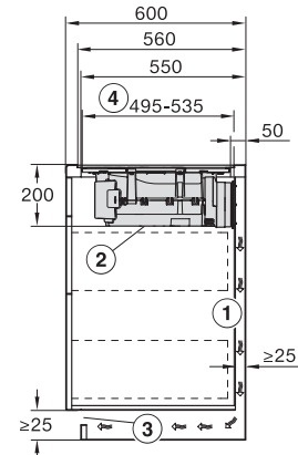
KMDA7272-1FL, KMDA7473-1FL/FL MattFinish, KMDA7272FL, KMDA7473FL - Side view flush, Plug&Play
