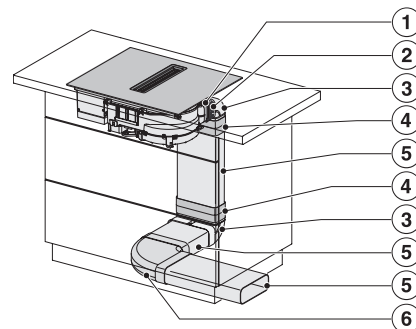
KMDA5649FL, KMDA5649FR, KMDA5649FL MattFinish – Installation variant 3 Basis
