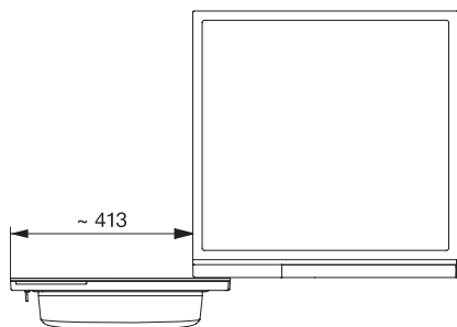
T2 with glass door, fascia 17 degree, measures in mm
