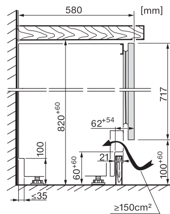
KWTUS7096E, Built-under, side view (installation drawings)
