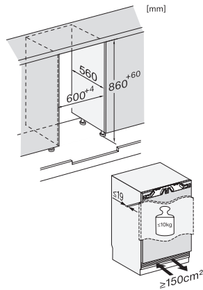
KU7135C, FNUS7140C, Built-under, installation diagram, niche dimensions
