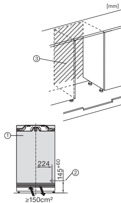
KU7016D, KU7015D, KU7035D, KU7135C, FNUS7140C, Built-under, installation drawing
