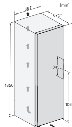
FNS4382D, FNS4382E, installation sketch (footnote*) (installation drawings)
