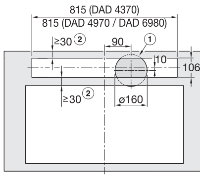
DAD4370, DAD4870, DAD4970, DAD6880, DAD6980, Installation drawings
