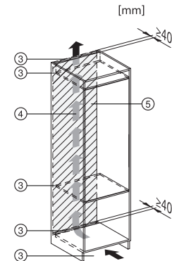
K7313D, K7313F, K7314E, K7314F, K7303F, K7303D, K7304F, K7304E, installation (footnote*) (installation drawings)
