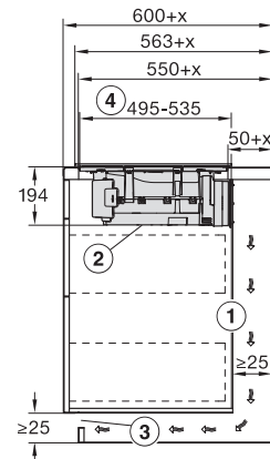
KMDA7272-1FR, KMDA7473-1FR, KMDA7272FR, KMDA7473FR – Side view lying on top+X, Plug&Play
