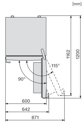
KF4472CD, top view (installation drawings)
