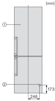
KF4472CD, connection sketch (footnote*) (installation drawings)
