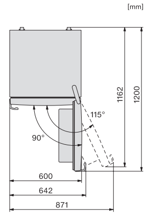
KF4472CD, top view (installation drawings)
