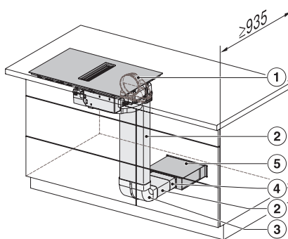
KMDA7272-1FL/FR, KMDA7473-1FL/FL MattFinish/FR, KMDA7272FL/FR, KMDA7473FL/FR – Installation variant 3 Basis
