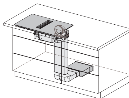
KMDA7272-1FL/FR, KMDA7473-1FL/FL MattFinish/FR, KMDA7272FL/FR, KMDA7473FL/FR – Installation variant 12 Exhaust air
