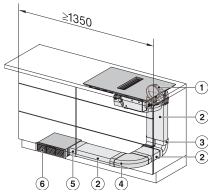
KMDA7272-1FL/FR, KMDA7473-1FL/FL MattFinish/FR, KMDA7272FL/FR, KMDA7473FL/FR – Installation variant 5 Circulating air
