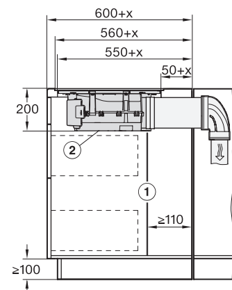
KMDA7473-1FL, KMDA7473-1FL MattFinish – Side view flush+X
