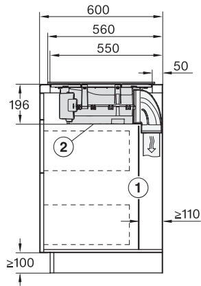
KMDA7272-1FL, KMDA7473-1FL/FL MattFinish, KMDA7272FL, KMDA7473FL – Side view lying on top
