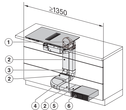
KMDA7272-1FL/FR, KMDA7473-1FL/FL MattFinish/FR, KMDA7272FL/FR, KMDA7473FL/FR – Installation variant 4 Circulating air
