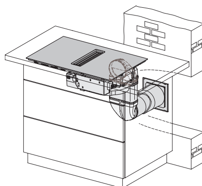
KMDA7272-1FL/FR, KMDA7473-1FL/FR, KMDA7473-1FL MattFinish, KMDA7272FL/FR, KMDA7473FL/FR, Exhaust air
