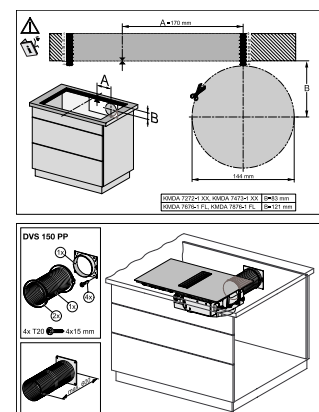
Installation plan DVS150PP
