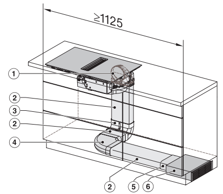
KMDA7272-1FL/FR, KMDA7473-1FL/FL MattFinish/FR, KMDA7272FL/FR, KMDA7473FL/FR – Installation variant 13 Circulating air
