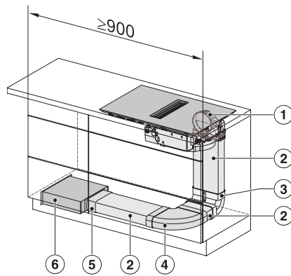
KMDA7272-1FL/FR, KMDA7473-1FL/FL MattFinish/FR, KMDA7272FL/FR, KMDA7473FL/FR – Installation variant 14 Circulating air
