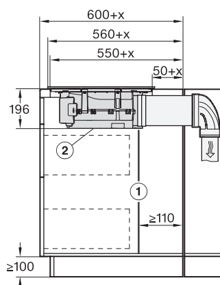
KMDA7473-1FL, KMDA7473-1FL MattFinish – Side view lying on top+X
