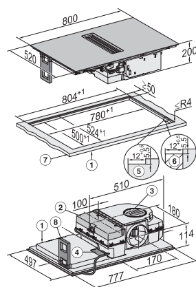
KMDA7473-1FL MattFinish – flush
