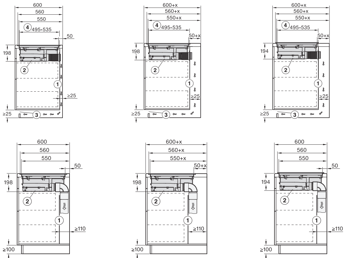
KMDA5649FL, KMDA5649FR, KMDA5649FL MattFinish – Installation variant 10 Exhaust air
