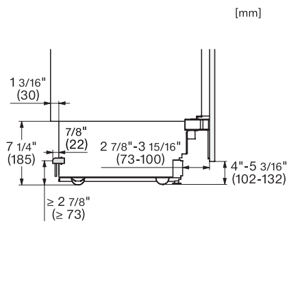
KFMC3632R+L, KFMC3642R+L, KFMC3836R+L, KFMC3834R+L, KFMC3858FD, MasterCool III, Side-view bottom, installation (drawing)
