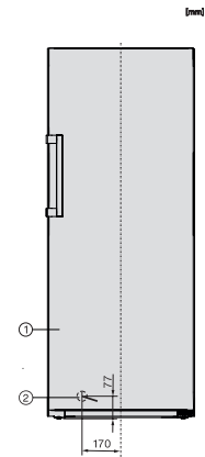
FN4748C, FN4748D, installation (footnote*) (installation drawings)
