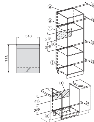
installation H7000 XL-55 CH, installation drawing
