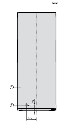
FN4849D, installation (footnote*) (installation drawings)
