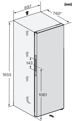
FN4849D, installation sketch (footnote*) (installation drawings)
