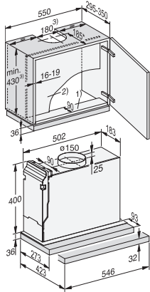
DAS2520, DAS4520, Installation drawings
