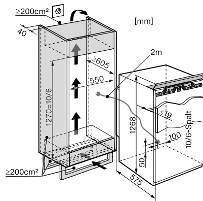
K34543-55 iF, K34543-55iF-1 (installation drawings)
