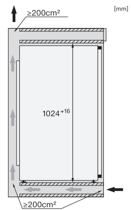
K7237D, K7238D, K7233E, K7234E, side view (installation drawings)
