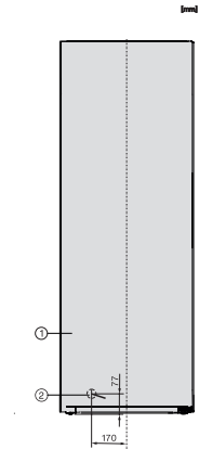
FN4879D, installation (footnote*) (installation drawings)
