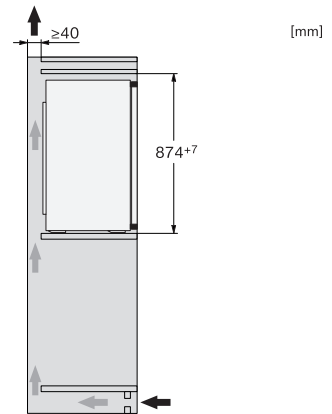
K7113D, K7113F, K7114E, K7103F, K7103D, K7104E, side view
