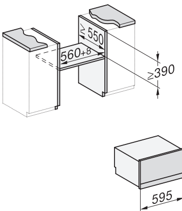
built-in DGD build-under, installation drawing
