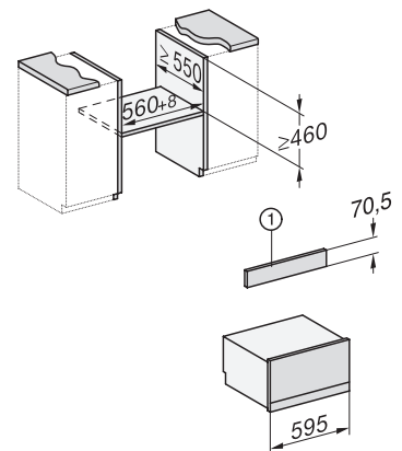
built-in DGD 450 build-under, installation drawing
