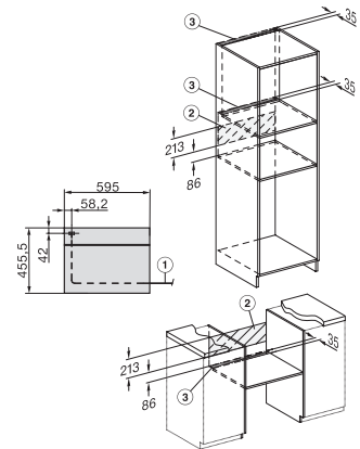
H7x4xB/BP/BPX, H2840B, installation drawings
