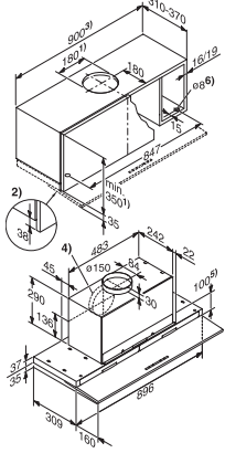
Installation drawings DA 3598, DA 3598 EXT
