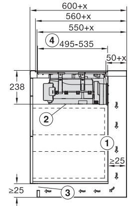
KMDA7676-1FL, KMDA7876-1FL, KMDA7676FL, KMDA7876FL – Side view flush+X, Plug&Play
