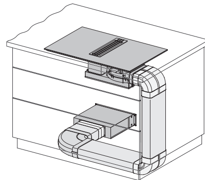
KMDA 7774, built-in version (Installation drawing)
