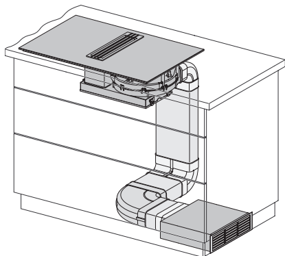
KMDA 7774, Built-in version 1 (Installation drawing)
