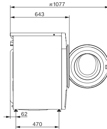
W1 drawing, fascia 5 degree, measures in mm
