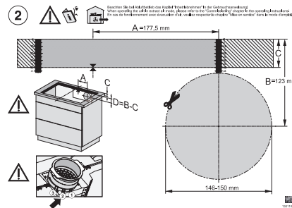
KMDA7272-1FL/FR, KMDA7473-1FL/FR – surface installation, 21 cm, drilling template
