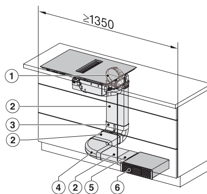
KMDA7272-1FL/FR, KMDA7473-1FL/FR, KMDA7272FL/ FR, KMDA7473FL/FR – Installation variant 4 Circulating air
