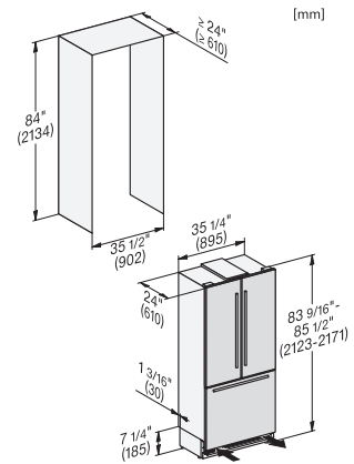
KFMC3642FD, KFMC3844FD, MasterCool III, PACS, with stainless steel front, integration
