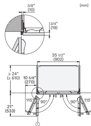
KFMC3642FD, KFMC3844FD, MasterCool III, PACS, with stainless steel front, top view
