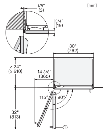
KFMC3632R+L, KFMC3836R+L, KFMC3834R+L, MasterCool III, PACS, with stainless steel front, top view
