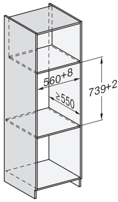
ESW7020, Installation drawings, XL combination niche height
