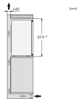
K7118D, K7128D, K7116E, K7126E, K7117D, K7127D, K7115E, K7125E, side view
